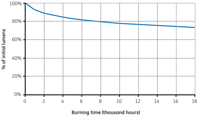
Lumen maintenance CMH G12 35W 4200K
